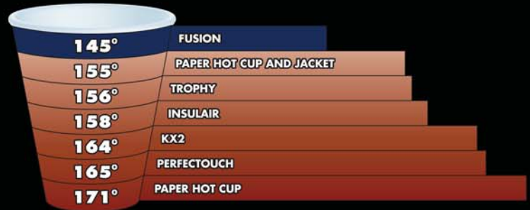
External Sidewall Temperature when beverage temperature measures 175°F
